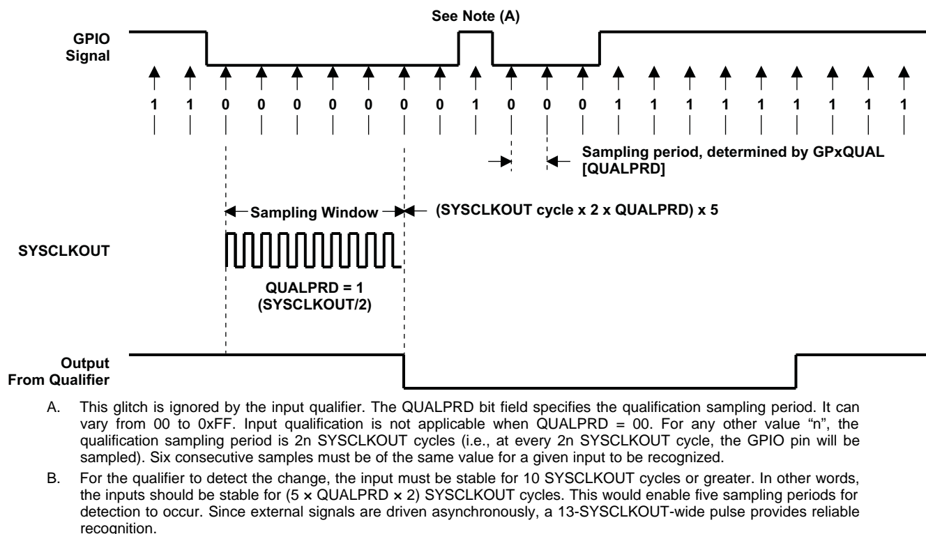
Figure 6-24. GPIO Input Qualifier – Example Diagram for QUALPRD = 1
