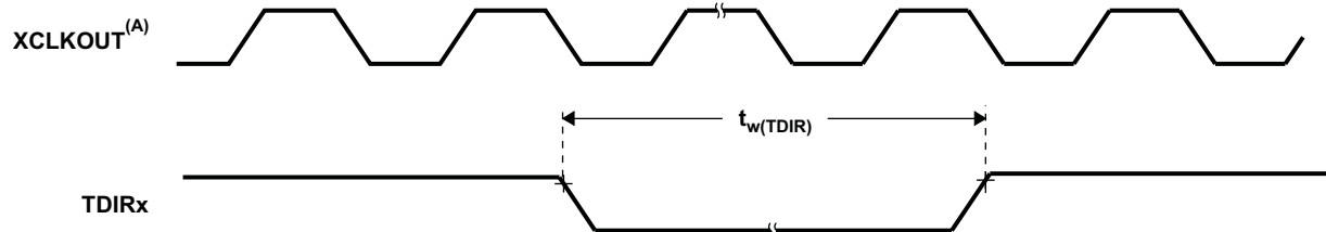
Figure 6-19. TDIRx Timing
