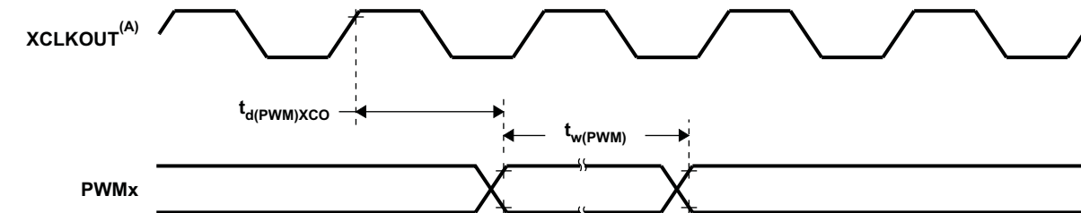
Figure 6-18. PWM Output Timing
